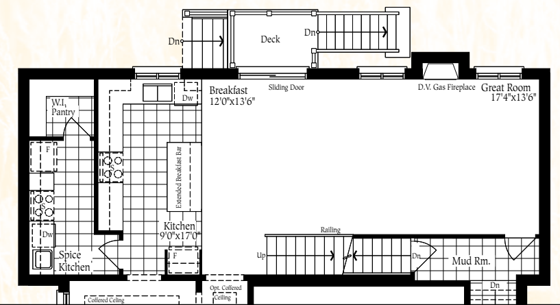
Optional Ground Floor Plan w/ Spice Kitchen Elevation A
